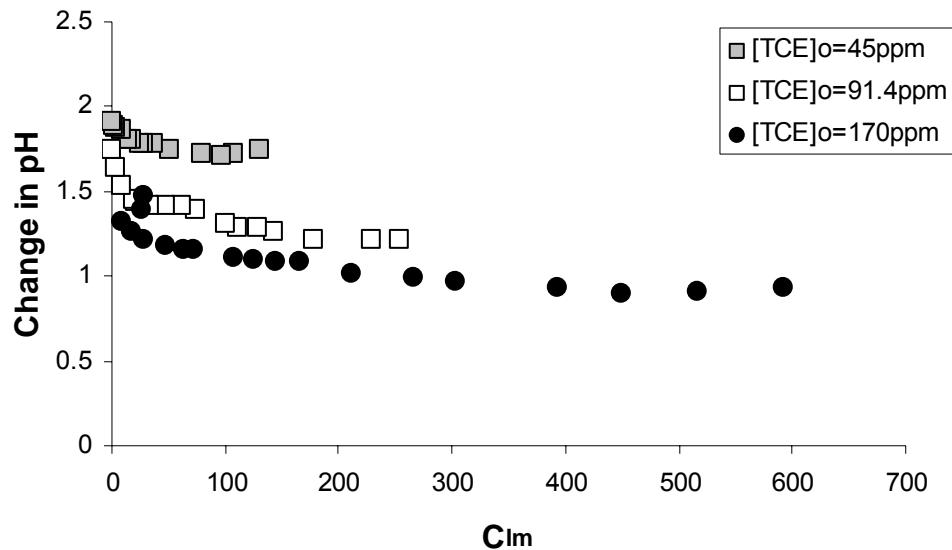
Figure 4.21 Effects of [TCE]_0 on Change in pH (effluent – Influent) vs. C_{1m} , [HCOOH^*] = 1 \text{ mM} ; Experiment #18: [TCE]_0 = 44.7 \text{ ppm} , Experiment #22: [TCE]_0 = 91.4 \text{ ppm} , Experiment #26: [TCE]_0 = 170 \text{ ppm} .
