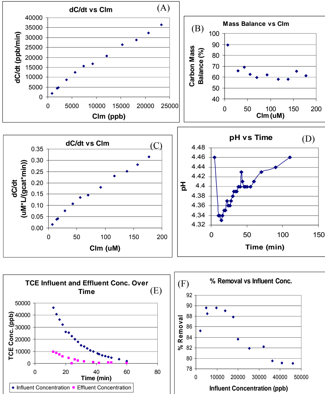
Figure B.23A Experiment #23 – pH = 4, [HCOOH*] = 10 mM, [TCE] 0 = 91.4 ppm (A) Degradation Rate vs. Clm (B) Carbon Mass Balance vs. Clm (C) Degradation Rate vs. Clm normalized (D) pH vs. Time [measured at the effluent] (E) Influent and Effluent TCE conc. vs. Time (F) % Removal vs. Influent conc.
