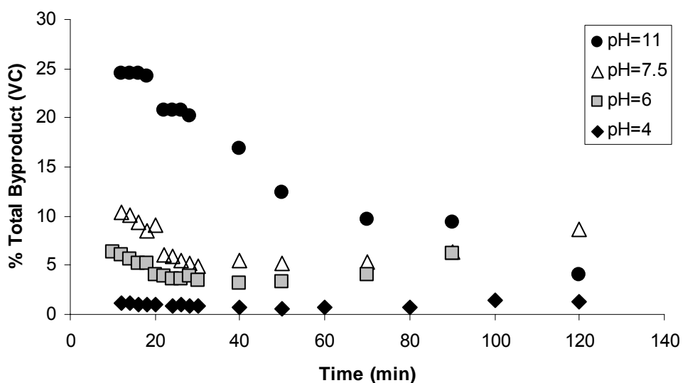
Figure 4.5 Effects of pH on vinyl chloride's percent of total byproducts produced vs. time, [\text{HCOOH}^*] = 4 \text{ mM} , [\text{TCE}]_0 = 25 \text{ ppm} ; Experiment #11: pH = 4, Experiment #13: pH = 6, Experiment #14: pH = 7.5, Experiment #16: pH = 11.
