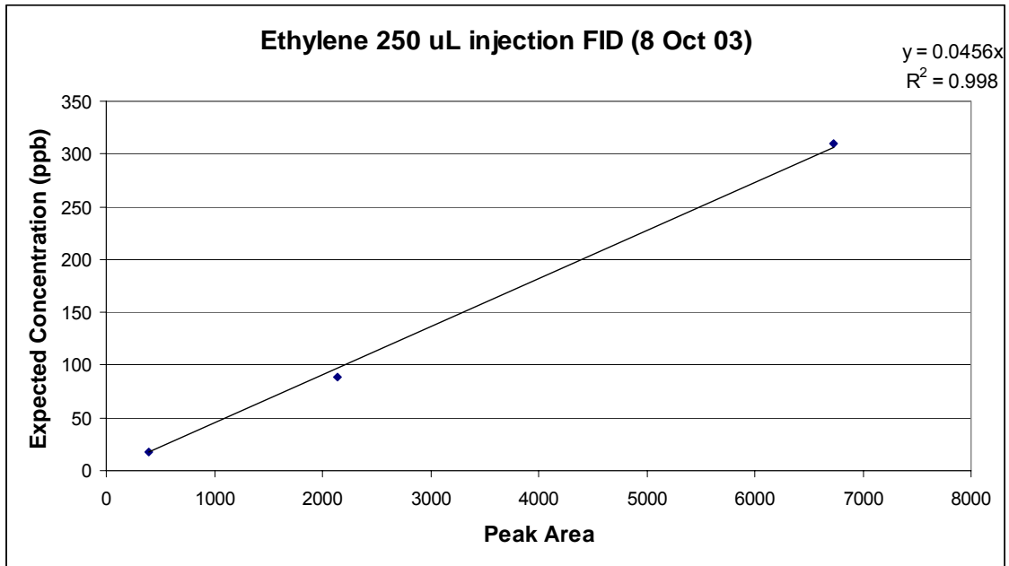
Figure A.6 Calibration curve: 250 \mu L ethylene injection, FID method
