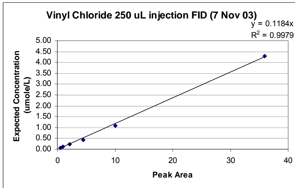
Figure A.7 Calibration curve: 250 µL vinyl chloride injection, FID method
