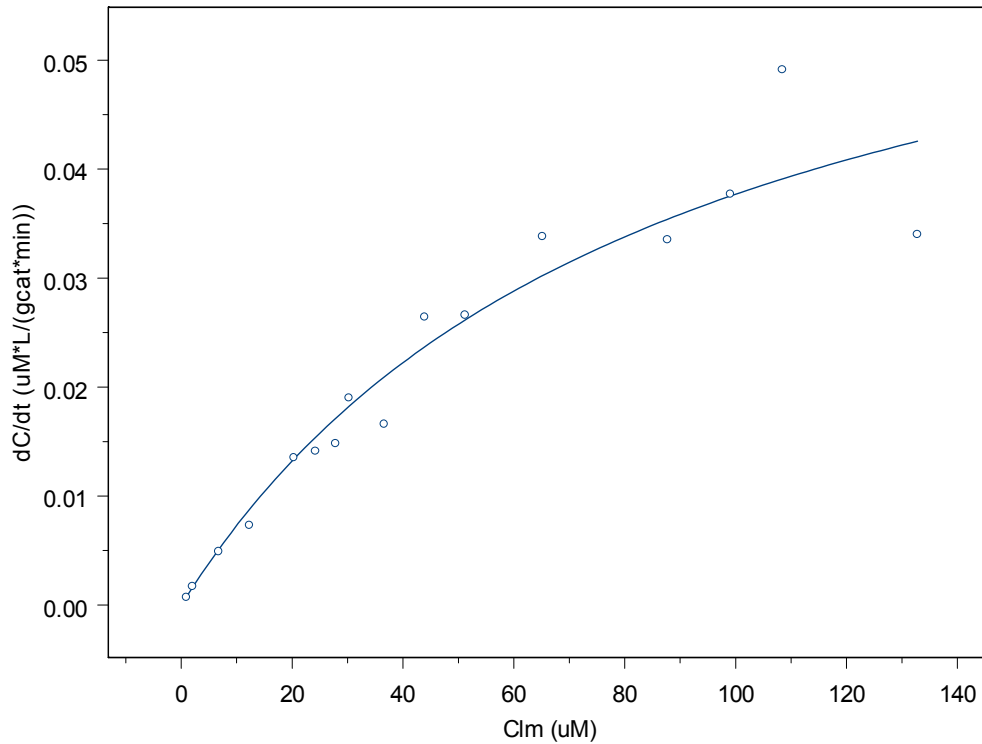
Figure C.7 Michaelis-Menten model fit to Experiment # 17 data: [TCE]_0 = 45 ppm, pH = 4 , [HCOOH^*] = 0.5 mM
