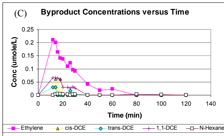
Figure B.11B Experiment #11 – pH = 4, [HCOOH*] = 4 mM, [TCE] 0 = 25 ppm cont. (A) Molar Byproduct Distribution vs. Time [measured at the effluent] (B) Ethane, Ethylene, VC Conc. vs. Time [measured at the effluent] (C) Ethylene, DCE, Hexane Conc. vs. Time [measured at the effluent]
