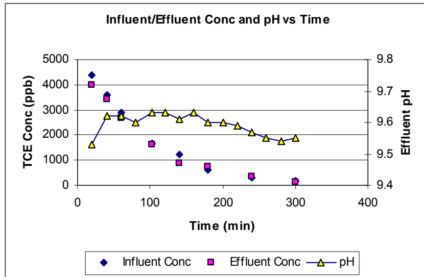
Figure B.2 Experiment #3 – pH = 7.75, [HCOOH*] = 1 mM, [TCE] 0 = 5 ppm, HRT = 4 min
