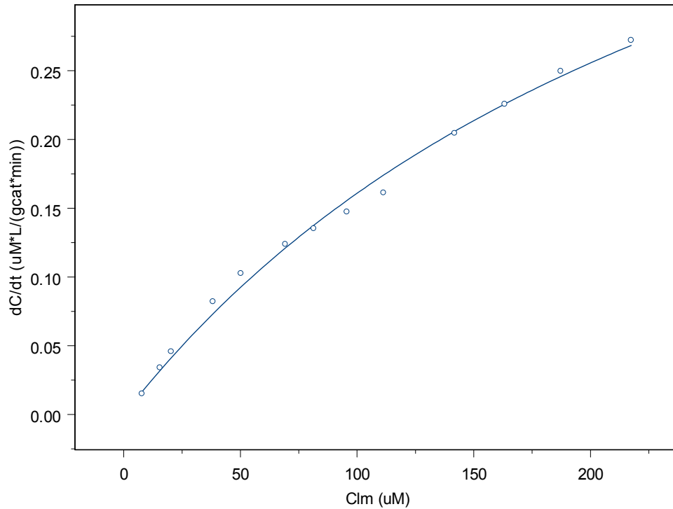
Figure C.11 Michaelis-Menten model fit to Experiment # 24 data: [TCE]_0 = 91.4 ppm, pH = 4 , [HCOOH^*] = 4 mM
