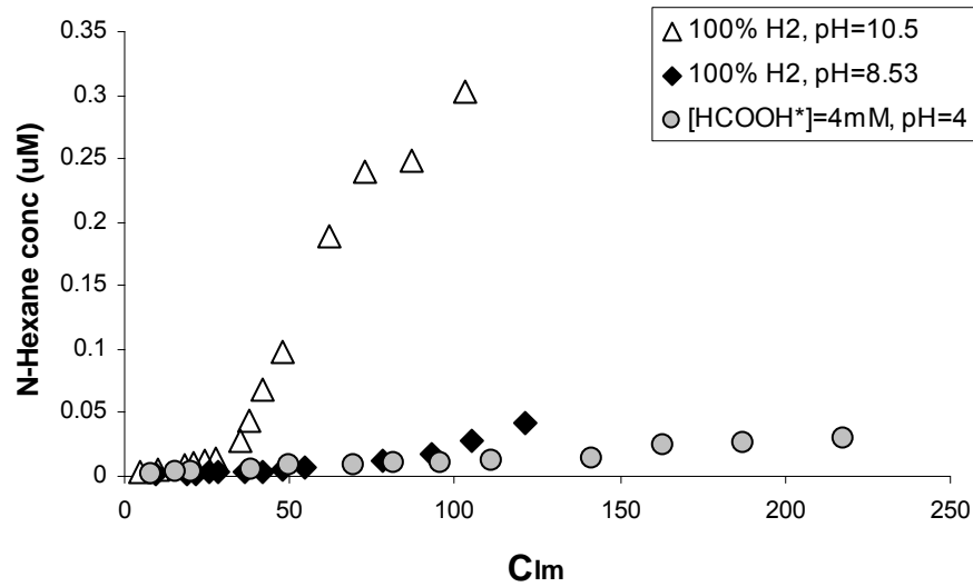
Figure 4.31 N-hexane concentration vs. C_{Im} , formate vs. hydrogen; Experiment #24: [HCOOH^*] = 4 \text{ mM} , \text{pH} = 4 , [TCE]_0 = 91.4 \text{ ppm} , Experiment #27: 100% H_2 , \text{pH} = 10.5 , [TCE]_0 = 44.7 \text{ ppm} , [TAPS] = 10 \text{ mM} , Experiment #28: 100% H_2 , \text{pH} = 8.53 , [TCE]_0 = 44.7 \text{ ppm} , [TAPS] = 10 \text{ mM} .
