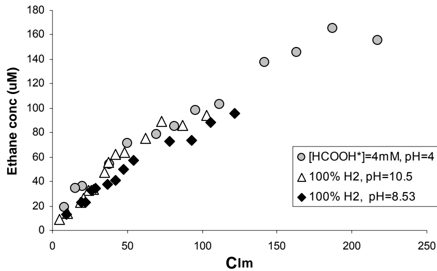
Figure 4.30 Ethane concentration vs. C_{Im} , formate vs. hydrogen; Experiment #24: [HCOOH^*] = 4 \text{ mM} , \text{pH} = 4 , [TCE]_0 = 91.4 \text{ ppm} , Experiment #27: 100% H_2 , \text{pH} = 10.5 , [TCE]_0 = 44.7 \text{ ppm} , [TAPS] = 10 \text{ mM} , Experiment #28: 100% H_2 , \text{pH} = 8.53 , [TCE]_0 = 44.7 \text{ ppm} , [TAPS] = 10 \text{ mM} .
