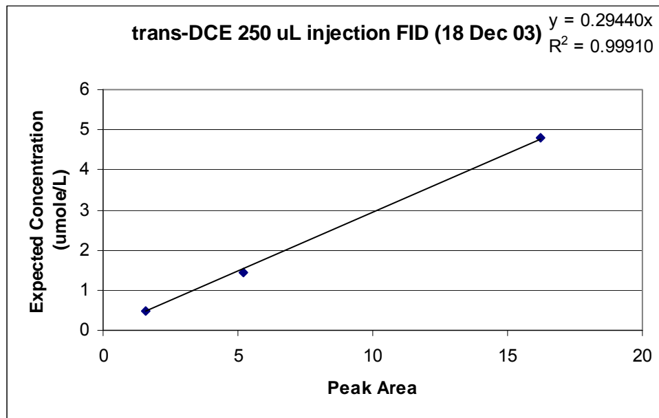
Figure A.9 Calibration curve: 250 µL trans-DCE injection, FID method
