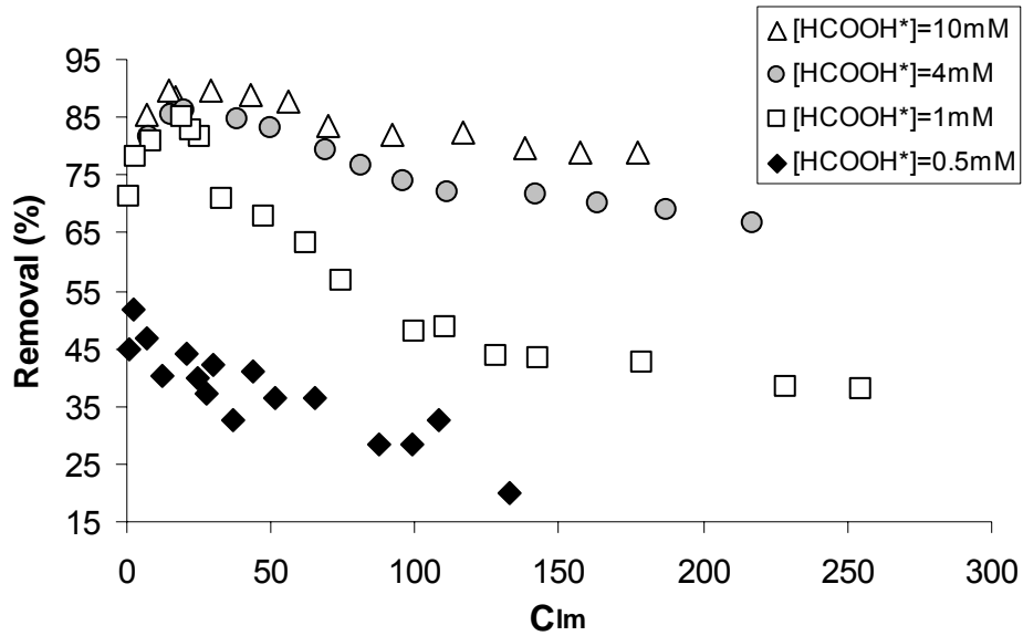
Figure 4.8 Effects of [HCOOH*] on TCE percent removal; Experiment # 17: [HCOOH*] = 0.5 mM, pH = 4, [TCE] 0 = 44.7 ppm, Experiment # 22: [HCOOH*] = 1 mM, pH = 4, [TCE] 0 = 91.4 ppm, Experiment #23: [HCOOH*] = 4 mM, pH = 4, [TCE] 0 = 91.4 ppm, Experiment #24: [HCOOH*] = 10 mM, pH = 4, [TCE] 0 = 91.4 ppm.
