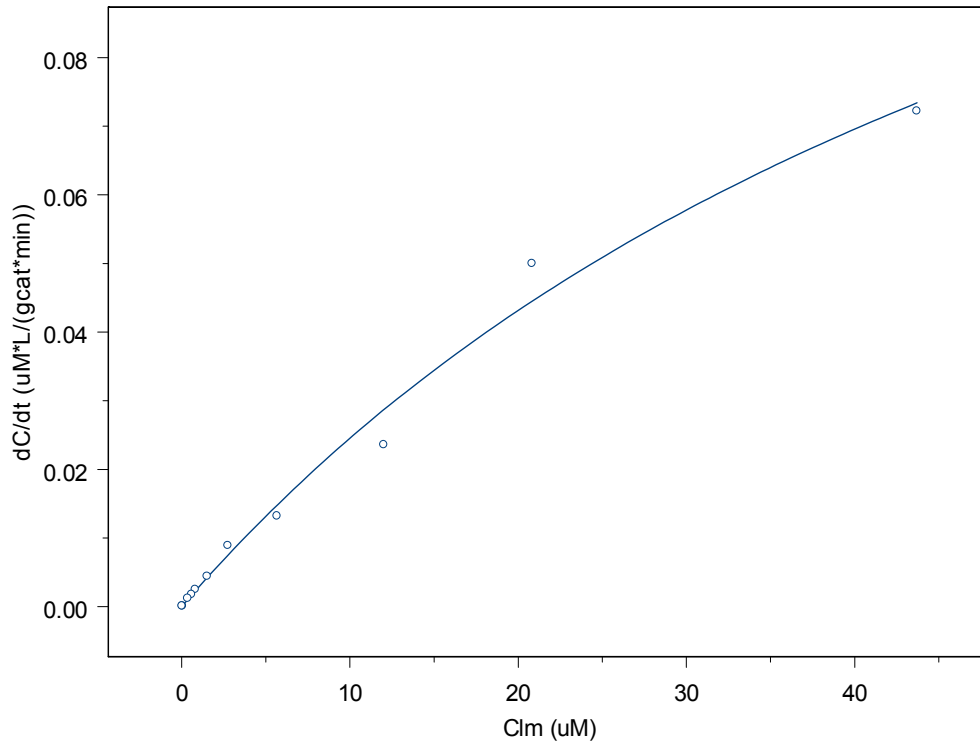
Figure C.1 Michaelis-Menten model fit to Experiment # 7 data: [TCE]_0 = 25 ppm, pH = 4 , [HCOOH^*] = 1 mM
