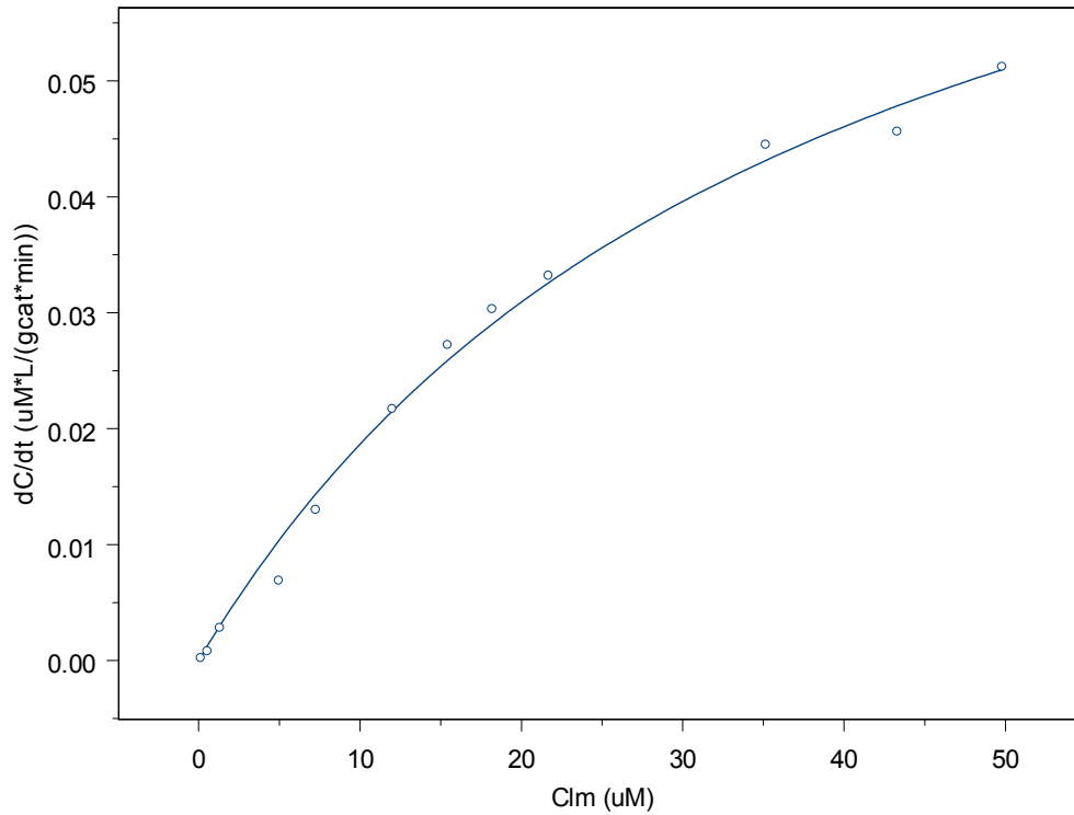
Figure C.4 Michaelis-Menten model fit to Experiment # 14 data: [TCE]_0 = 25 ppm, pH = 7.5 , [HCOOH^*] = 4 mM
