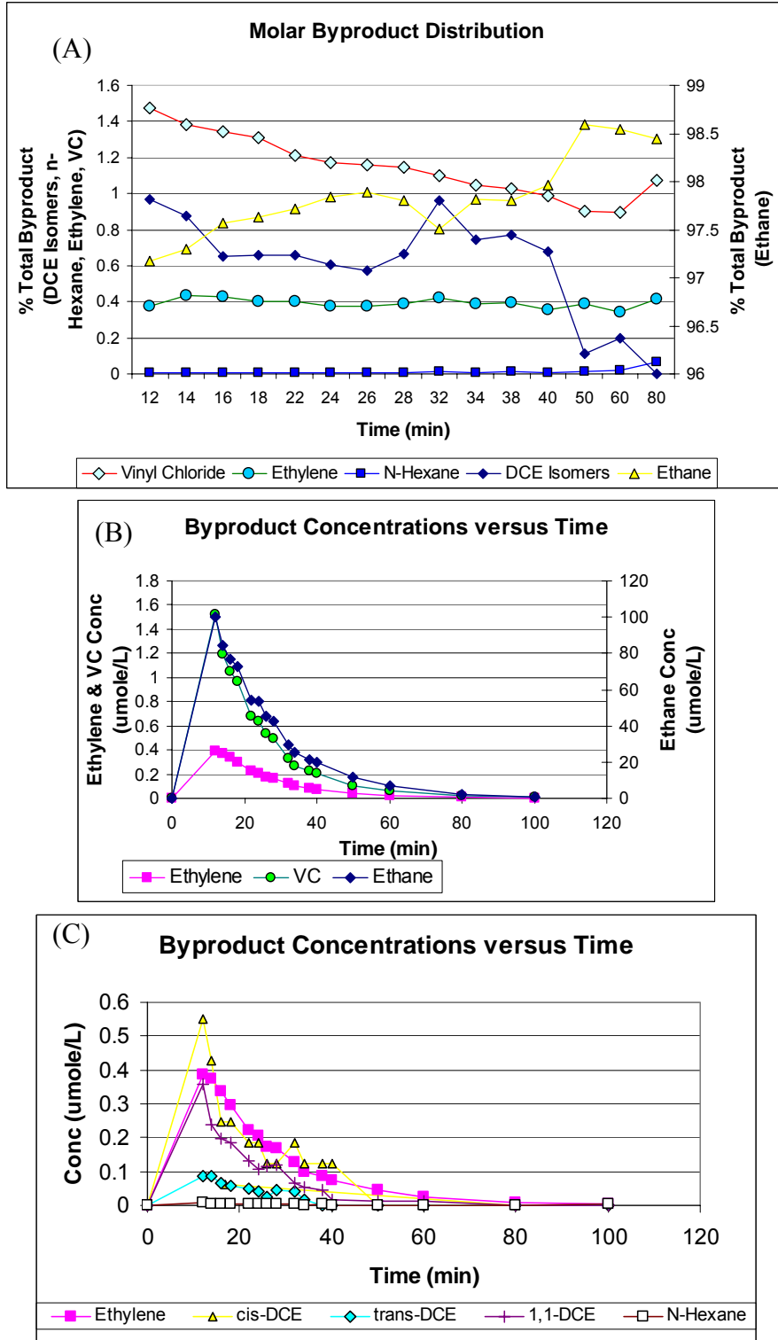
Figure B.19B Experiment #19 – pH = 4, [\text{HCOOH}^*] = 10 \text{ mM} , [\text{TCE}]_0 = 45 \text{ ppm} cont. (A) Molar Byproduct Distribution vs. Time [measured at the effluent] (B) Ethane, Ethylene, VC Conc. vs. Time [measured at the effluent] (C) Ethylene, DCE, Hexane Conc. vs. Time [measured at the effluent]
