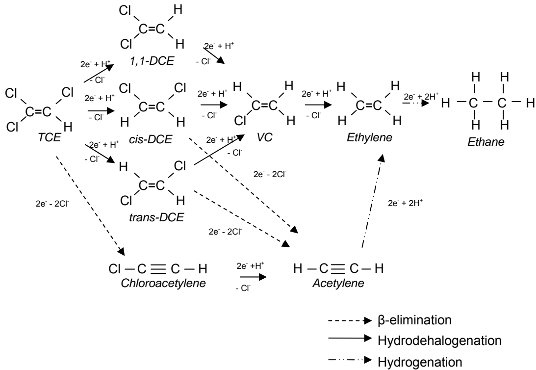
Figure 2.1 Hydrodehalogenation and reductive β-elimination pathways (Arnold and Roberts, 2000)
