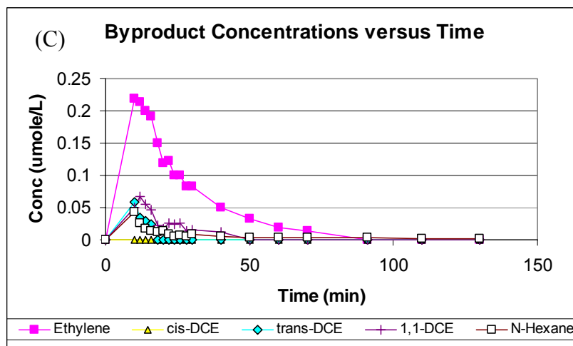
Figure B.12B Experiment #12 – pH = 5, [HCOOH^*] = 4 \text{ mM} , [TCE]_0 = 25 \text{ ppm} cont. (A) Molar Byproduct Distribution vs. Time [measured at the effluent] (B) Ethane, Ethylene, VC Conc. vs. Time [measured at the effluent] (C) Ethylene, DCE, Hexane Conc. vs. Time [measured at the effluent]
